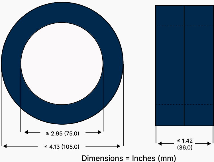
Dimensions = Inches (mm)
